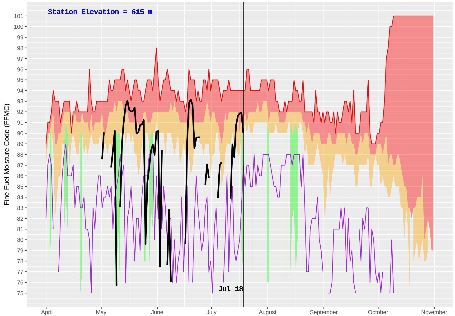
HIXON (187) : Historical (1976–2016) and Current (2018) Daily Fine Fuel Moisture Code (FFMC)
