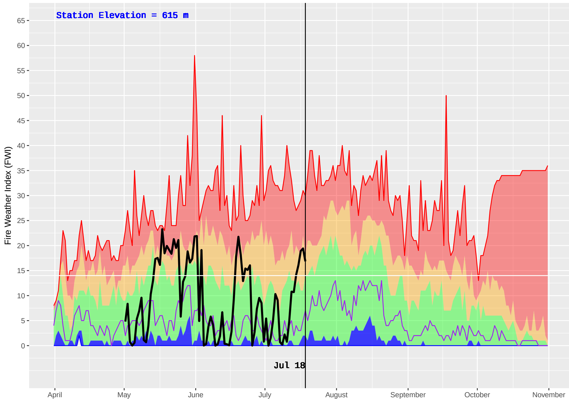
HIXON (187) : Historical (1976–2016) and Current (2018) Daily Fire Weather Index (FWI)
