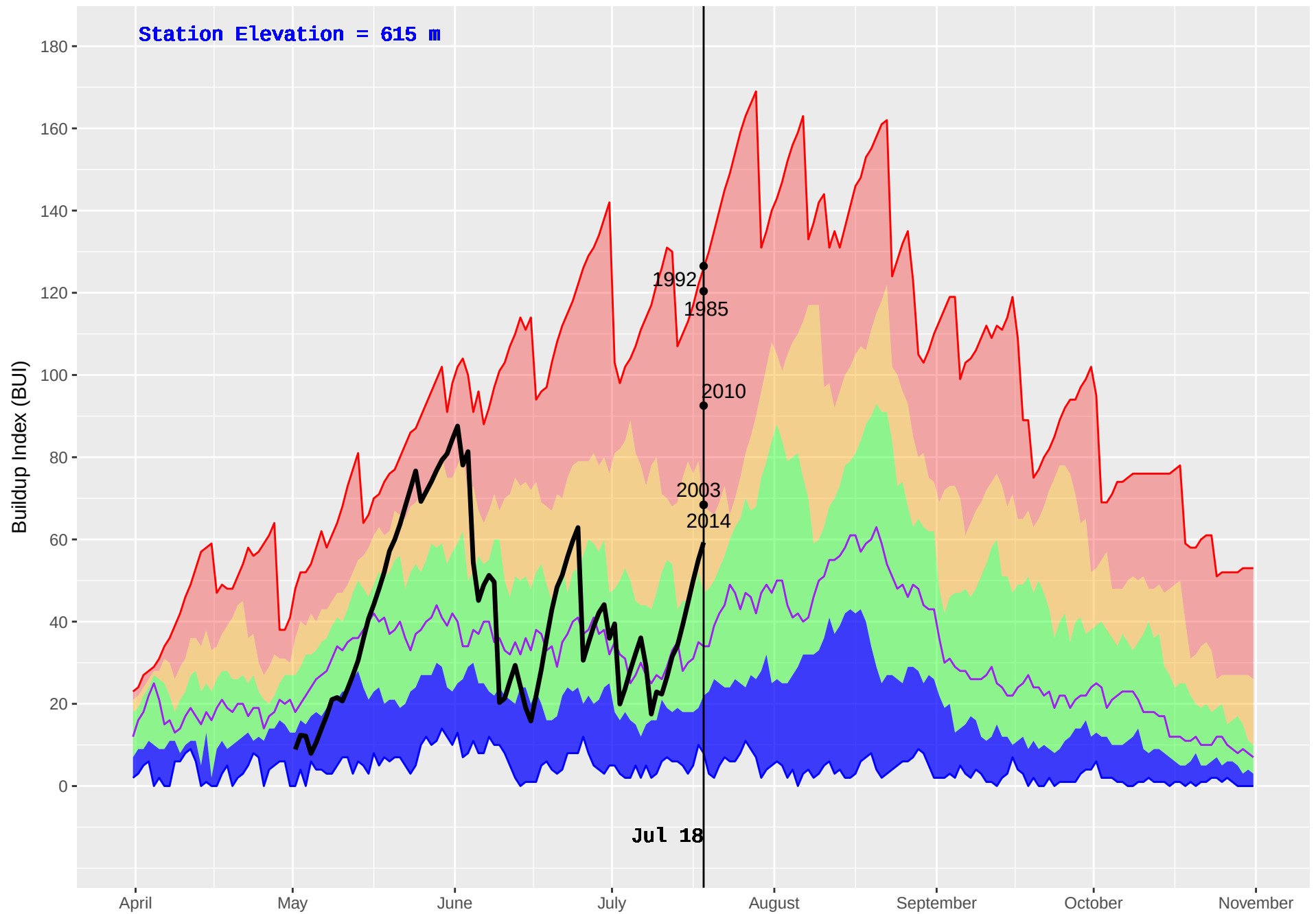
HIXON (187) : Historical (1976–2016) and Current (2018) Daily Buildup Index (BUI)
