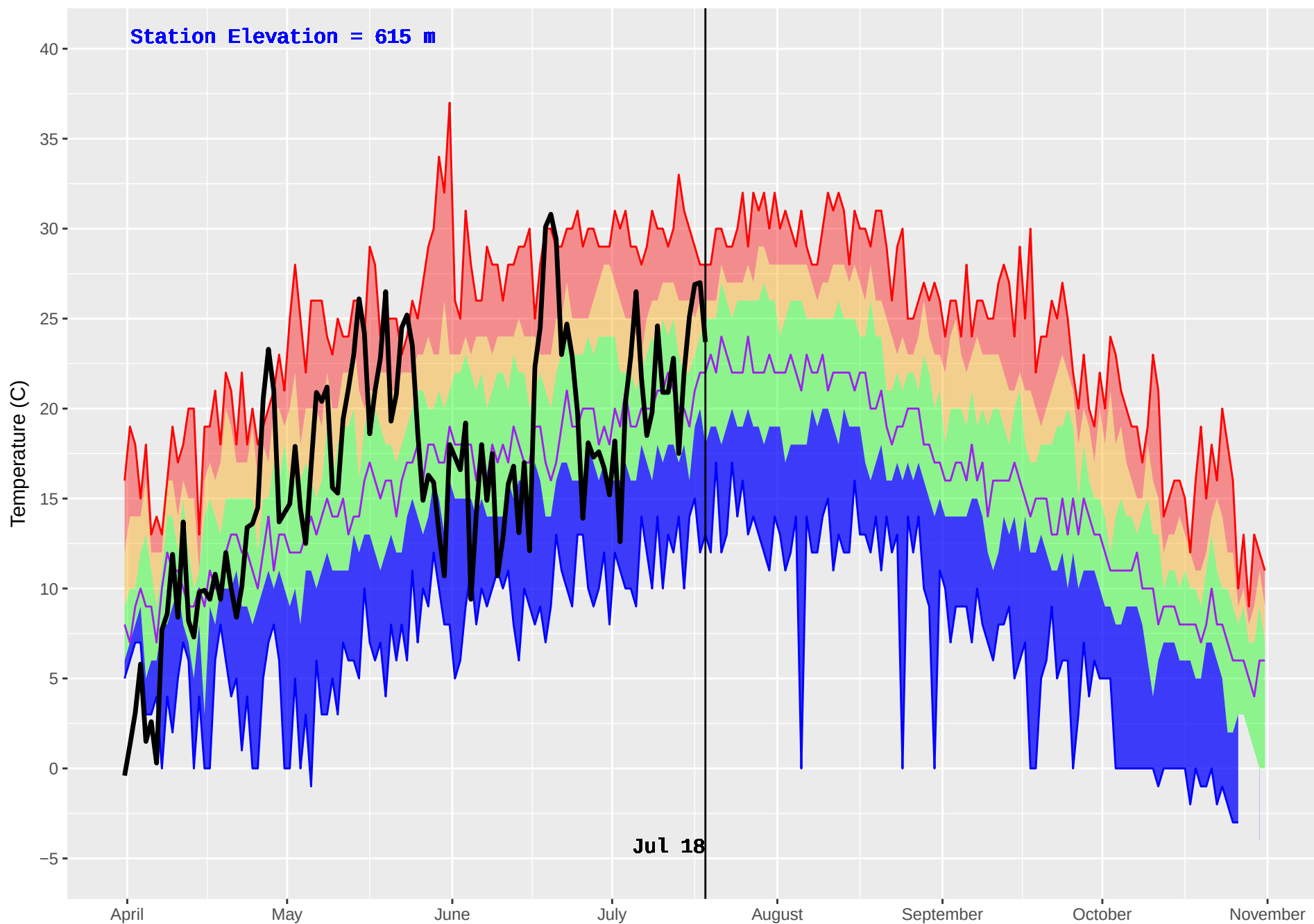
HIXON (187) : Historical (1976–2016) and Current (2018) Daily Temperature
