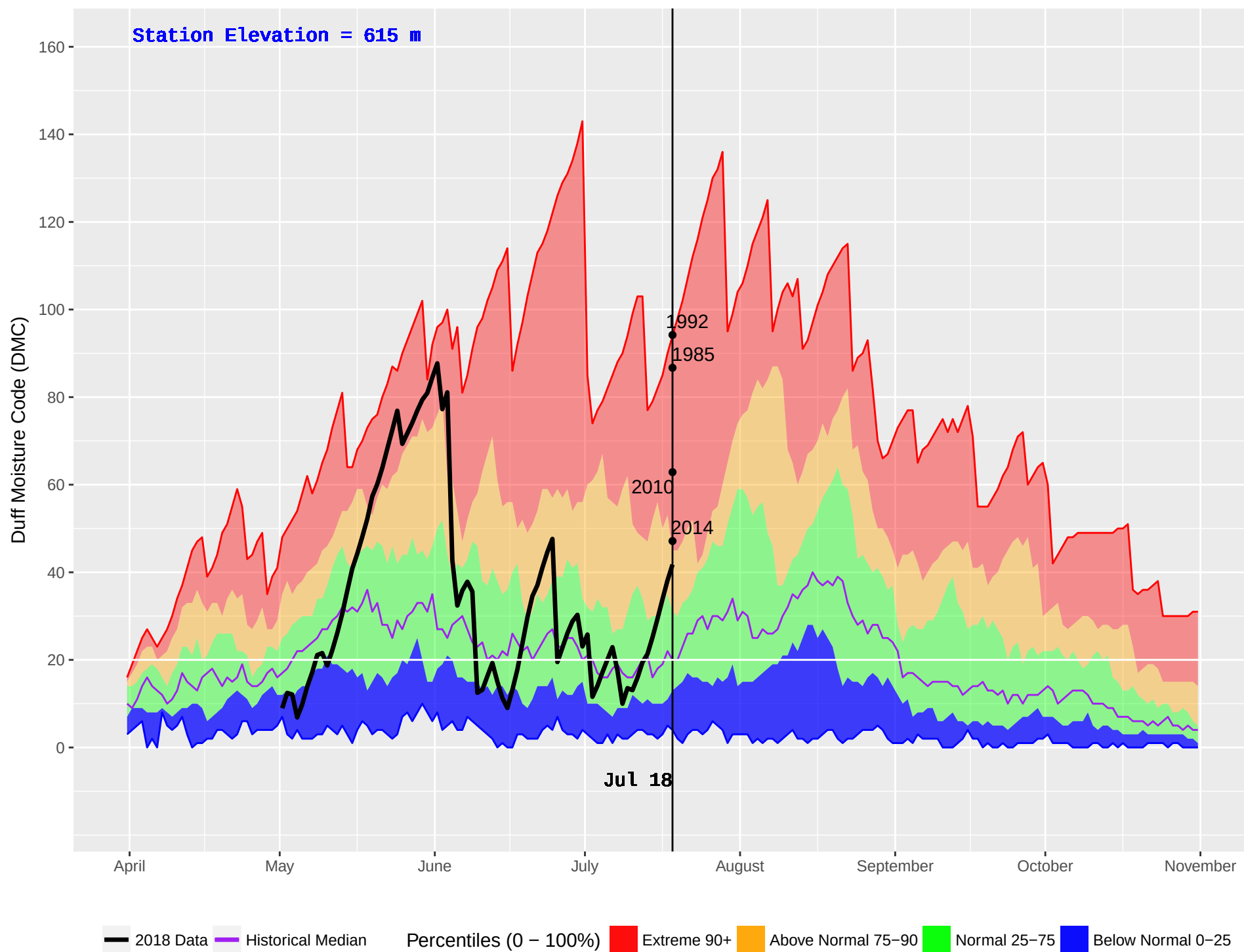
HIXON (187) : Historical (1976–2016) and Current (2018) Daily Duff Moisture Code (DMC)
